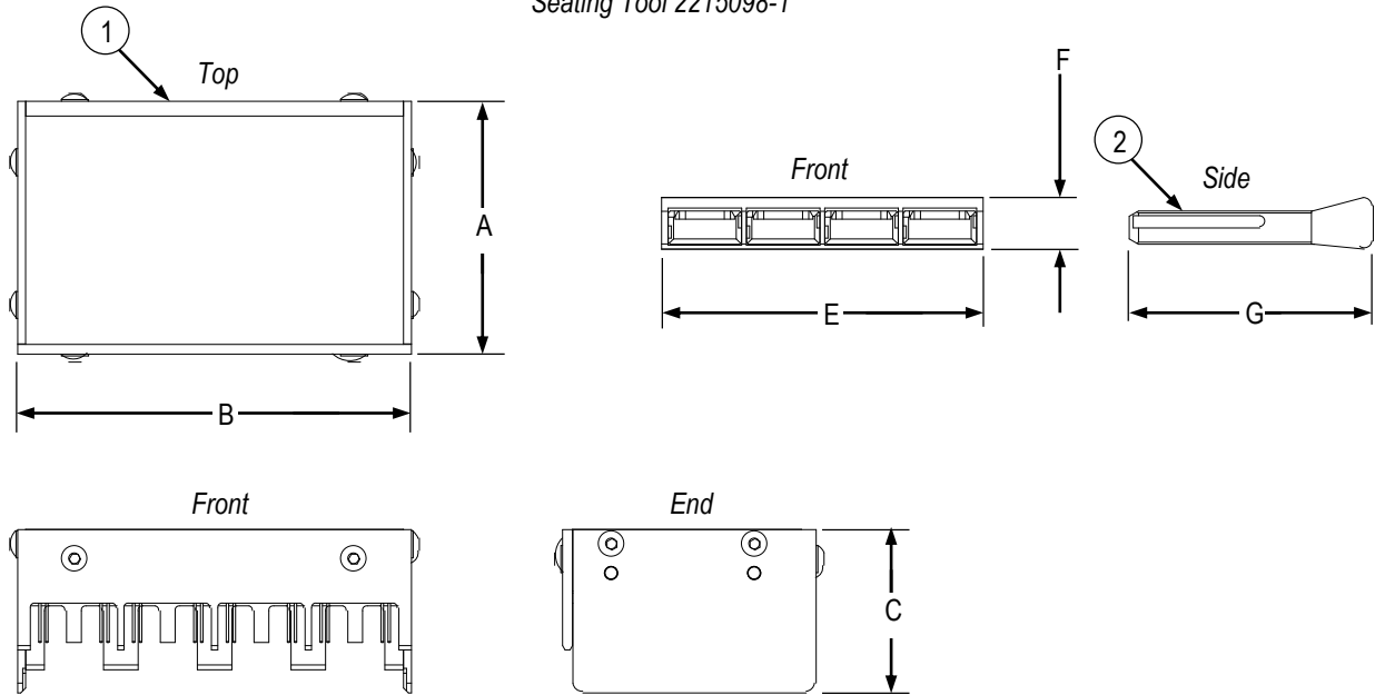
Seating Tool 2215098-1
