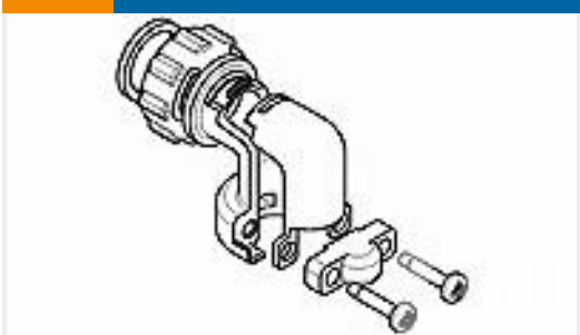
TE Part #1546347-2 R/A CABLE CLAMP KIT,SZ 11,CPC
