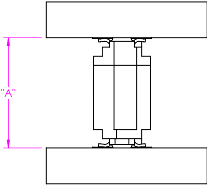
FIGURE 1 ERM6 MATED WITH ERF6
