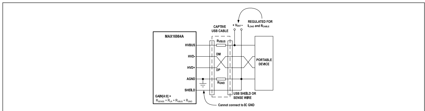
Figure 2. Remote Cable-Sense Diagram
