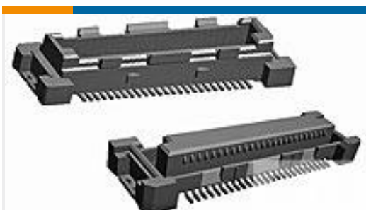
TE Part # 1-6123582-0 .6FHP10H,140,S,GIG,08/Sn,ST,NSYes
