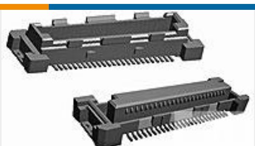
TE Part # 1-5353186-0 .6FHP06H,140,S,GIG,08/Sn,TR,NSYes
