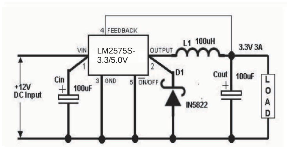
Typical Application of LM2575S For 3.3V,5.0V
