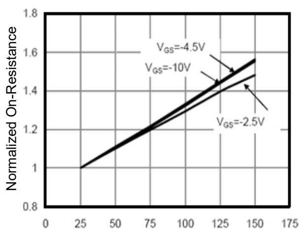
T_J -Junction Temperature( ^{\circ} C) Figure 6 Drain-Source On-Resistance
