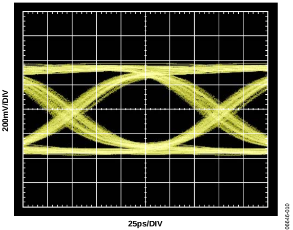
Figure 10. 6.5 Gbps Output Eye, 20 Inch FR4 Input Channel (TP3 from Figure 7)
