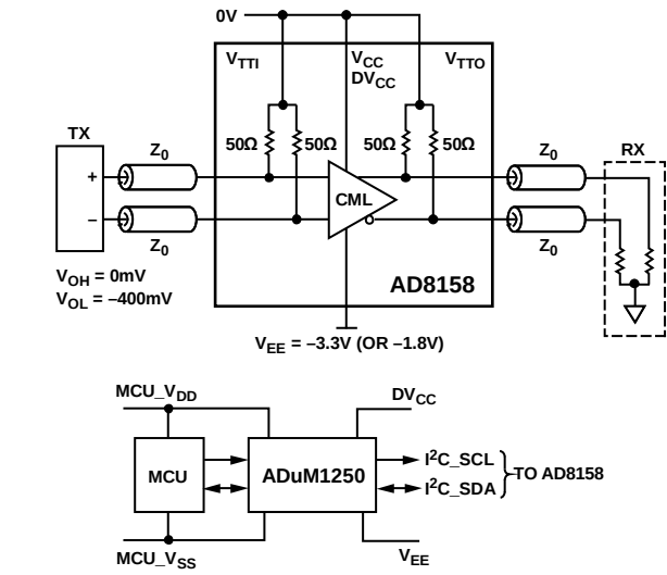
Figure 47. Multiple Supply Operation
