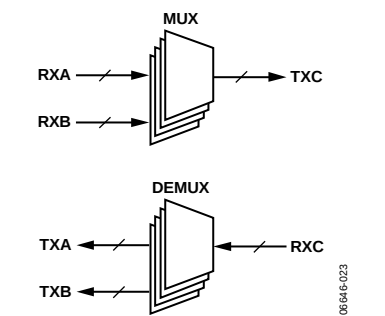
Figure 35. Mux/Demux Paths, Port A to Port C
