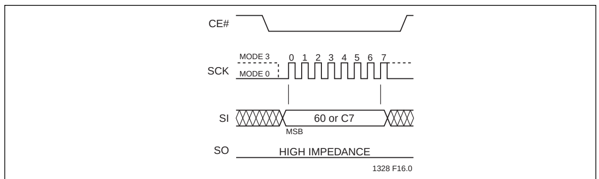
Figure 16: Chip-Erase Sequence
