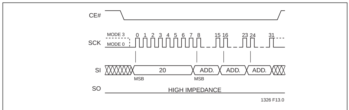
Figure 13: Sector-Erase Sequence
