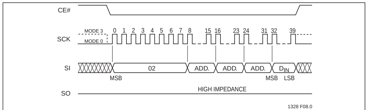
Figure 8: Byte-Program Sequence
