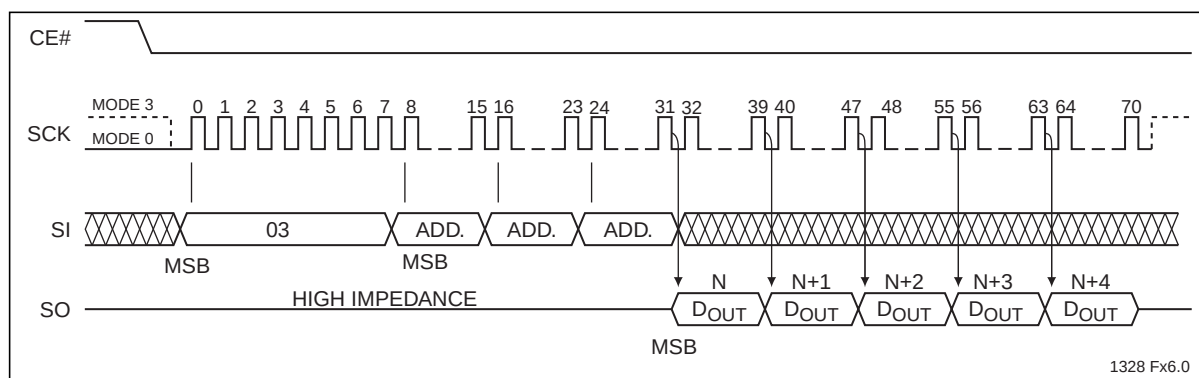
Figure 6: Read Sequence
