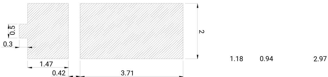
Recommended Solder Pad
