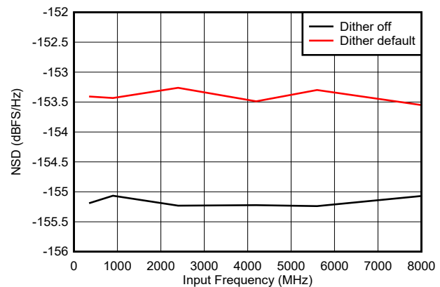
Figure 5-36. DES Mode: NSD vs Input Frequency
