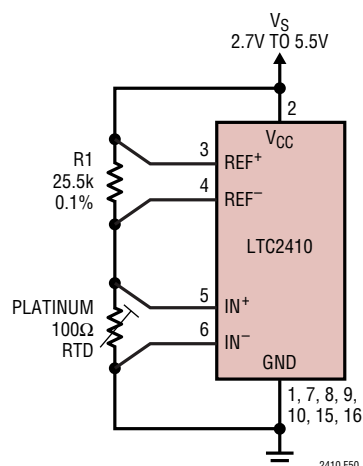
Figure 50. Remote Half Bridge Interface
