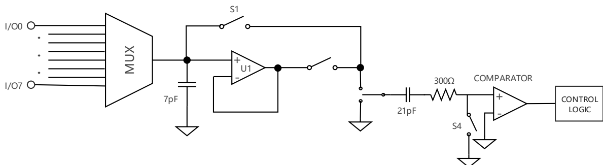
Figure 6 ADC input structure
