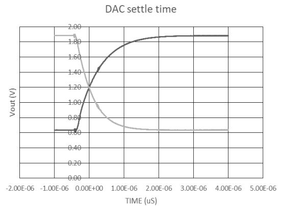
Figure 4 DAC settling time, output range = 0~Vref
