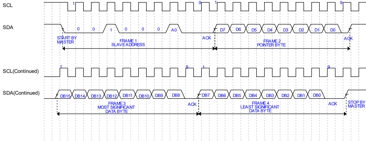
Figure 7 I 2 C Write
