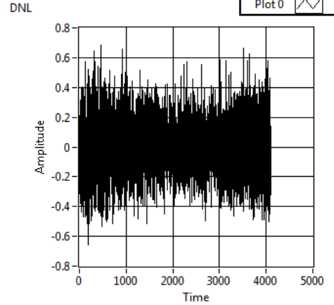
Figure 2. ADC DNL
