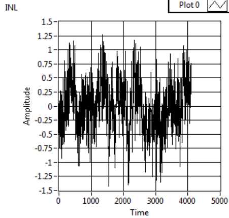
Figure 1. ADC INL
