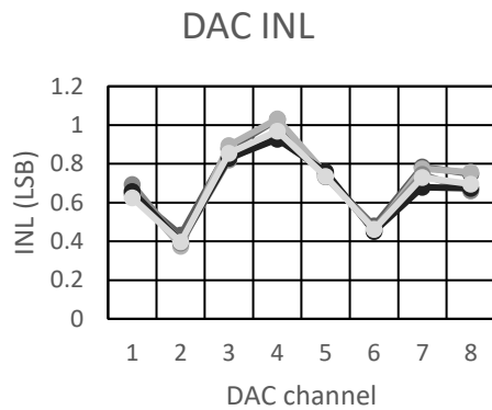
Figure 3 DAC INL
