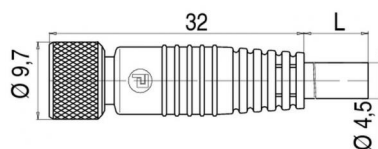
scale drawing
