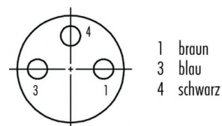
Contact Arrangement
