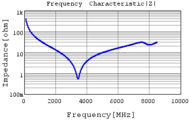
GCH1885C2A4R0CE01 |Z| DCOV, 25degC
