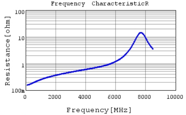
GCH1885C2A4R0CE01 R DCOV, 25degC
