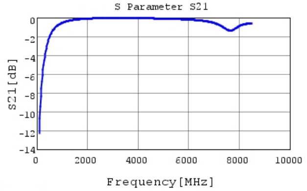
GCH1885C2A4R0CE01 S21 DCOV, 25degC
