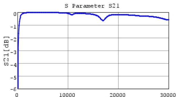
■ GJM0225C1C9R3BB01 S21 DCOV, 25degC
