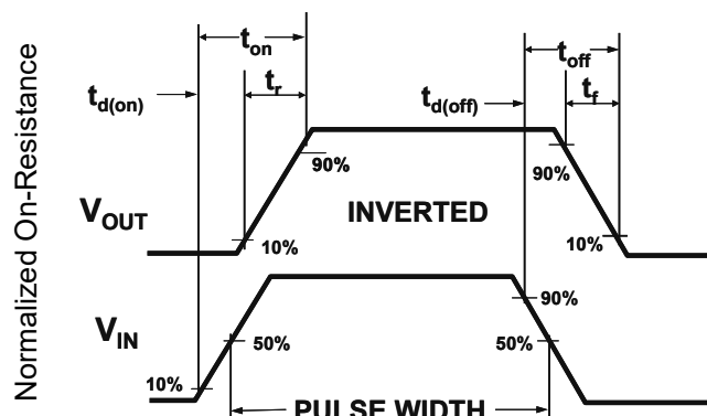
Figure 2: Switching Waveforms
