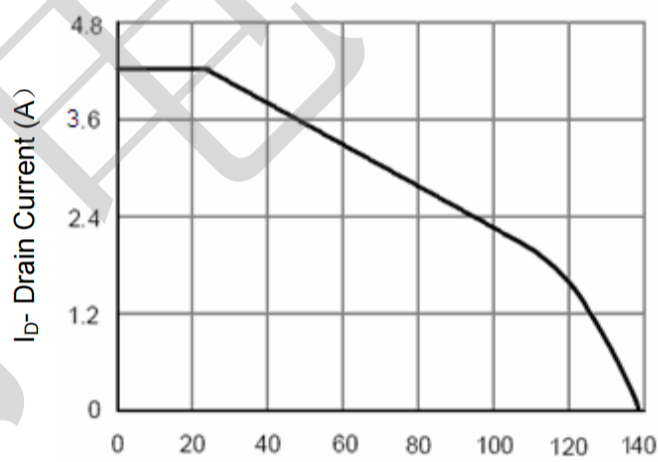
Figure 4 Drain Current
