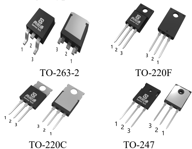
Figure 2 Package Types of SRC60R140BS
