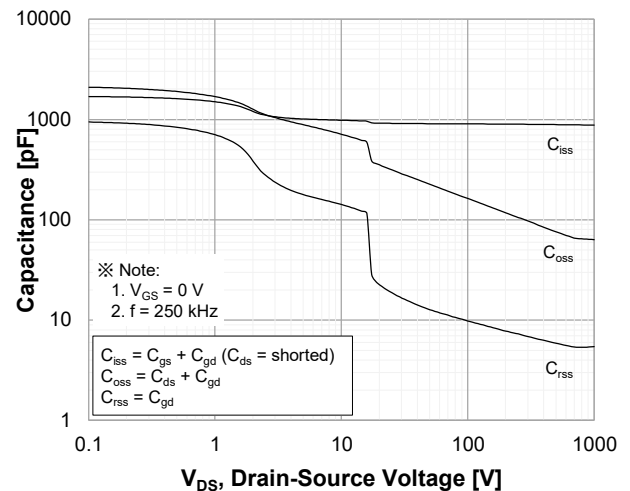
Figure 12. Capacitance Characteristics
