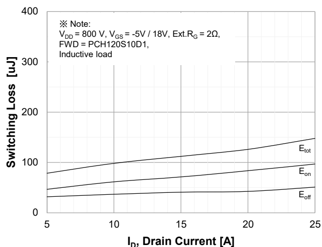
Figure 15. Typ. Switching Losses vs. Drain Current
