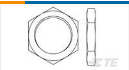
TE Part #1604196-1 NUT, JAM, 5/8-24, PKG QTY 100
