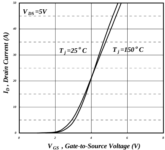
Fig 11. Transfer Characteristics
