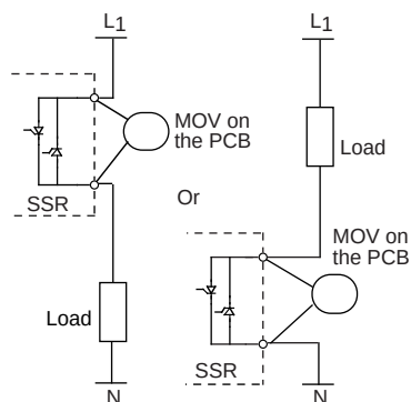
Figure 2 — LS relays
