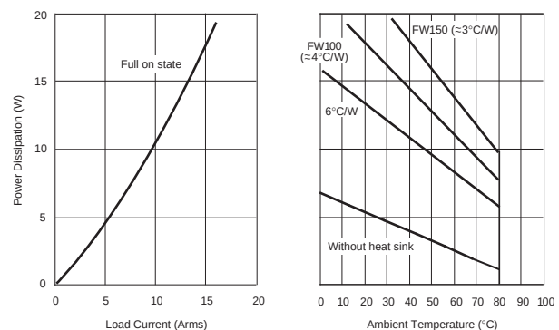
Figure 4 — LS relays
