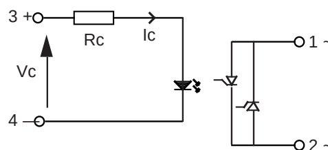
Figure 3 — LS relays
