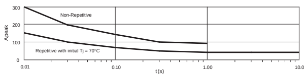
Figure 6c — LS60D22C relay
