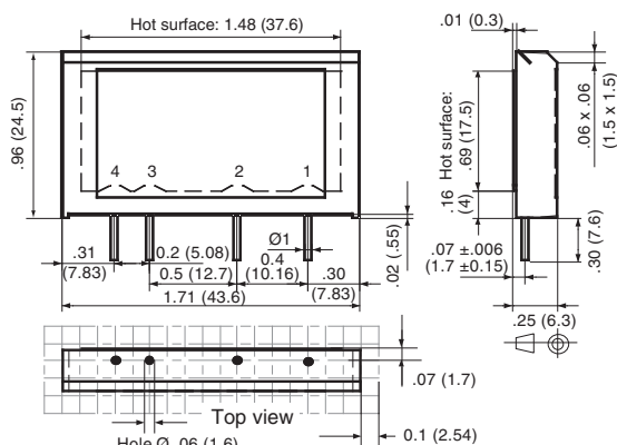
Figure 1 - LS relays; dimensions in inches (mm) (See Figure 12 for LS with HS1)
