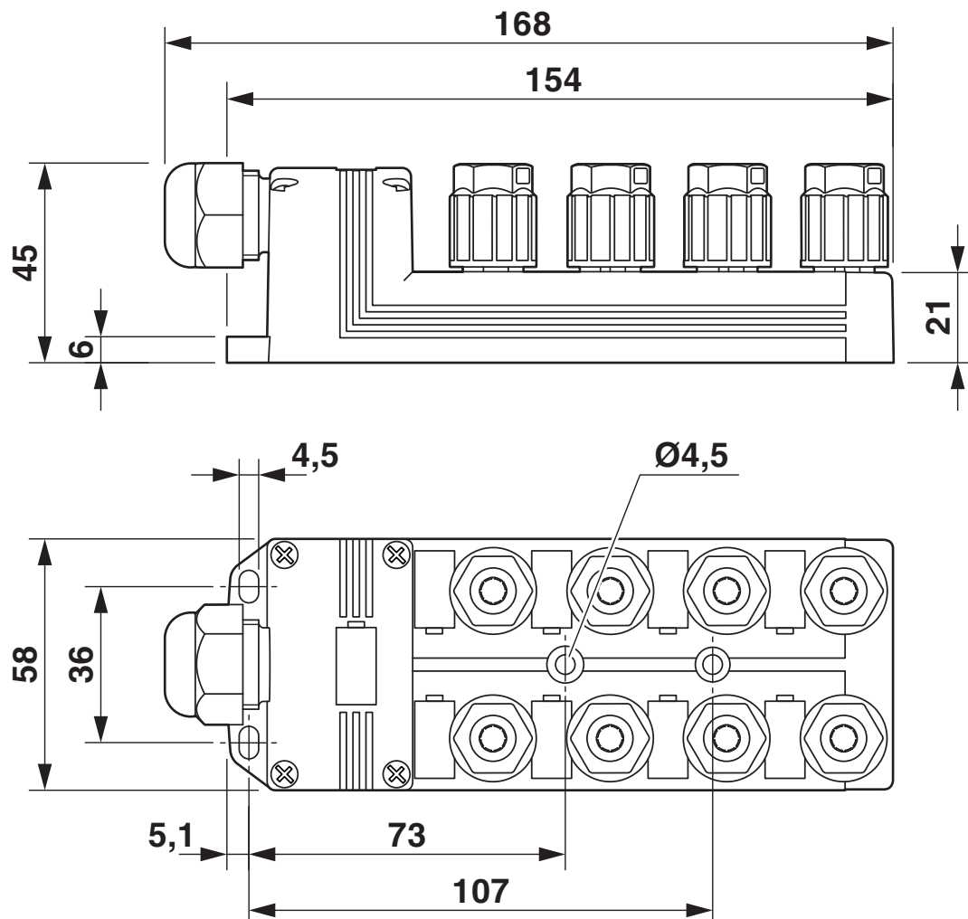
Dimensional drawing
