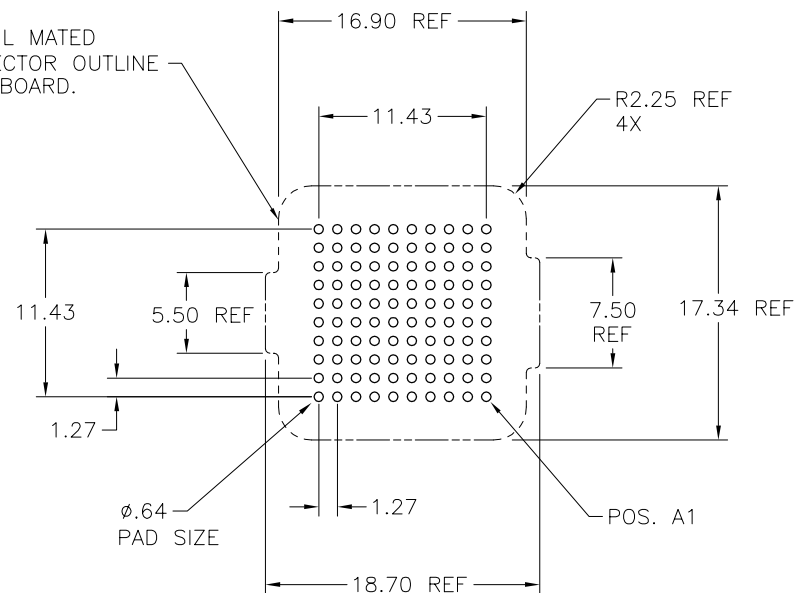
BOARD PATTERN
