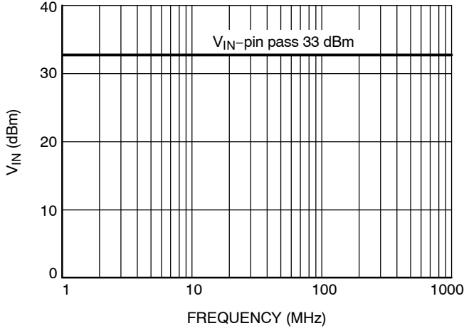
Figure 26. Typical V_{IN} -pin Susceptibility
