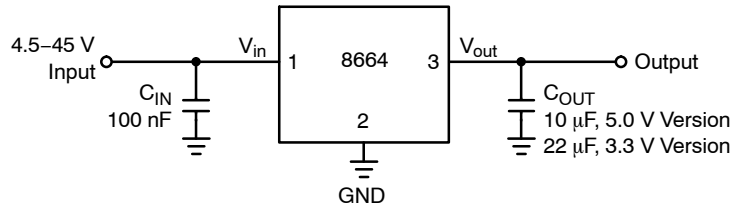
Figure 3. Applications Circuit
