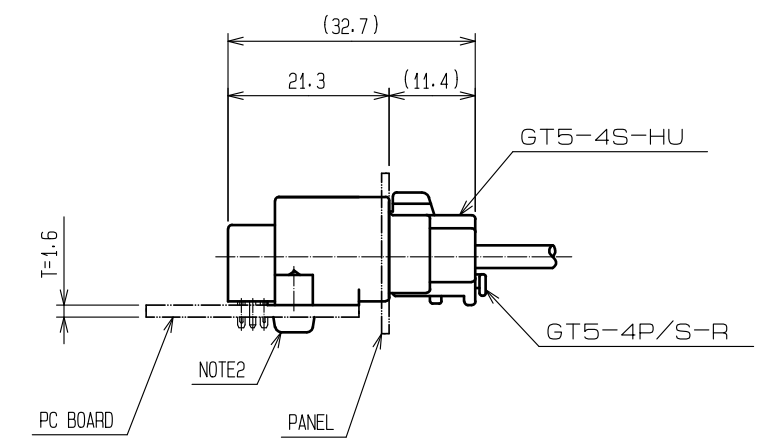
MATED CONNECTORS
