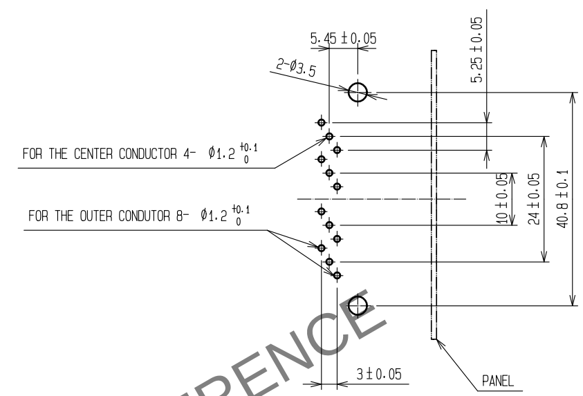
RECOMMENDED PC BOARD HOLE PATTERN
