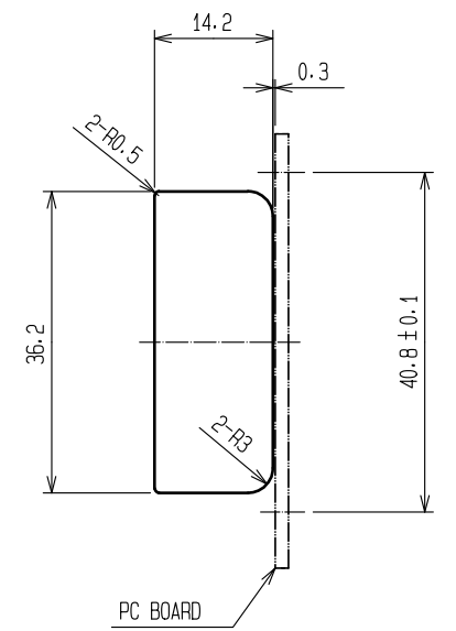
RECOMMENDED PANEL CUTOUT
