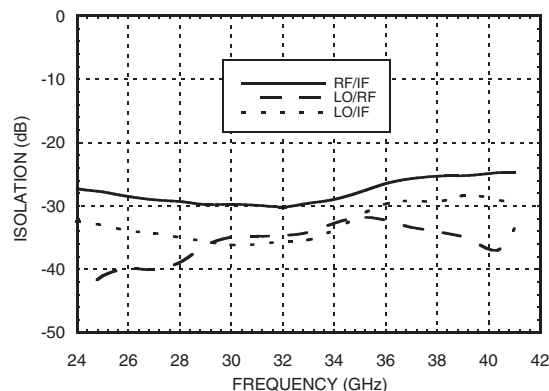
Isolation vs. Frequency @ LO +13 dBm
