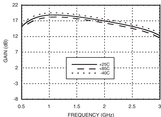
Gain*
