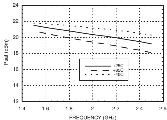
Output Psat*
