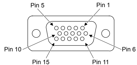
Figure 5-11 VGA connector
