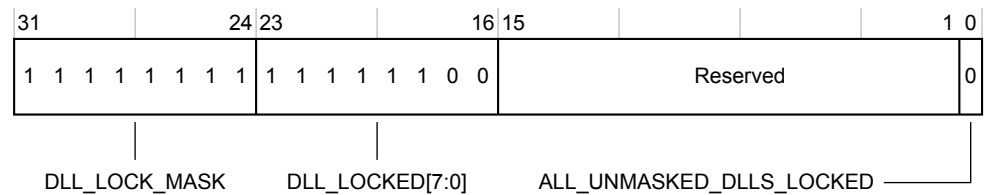
Figure 4-5 SCC_DLL Register bit assignments
