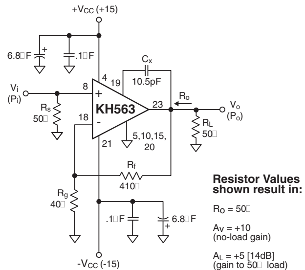
Figure 1: Test Circuit
