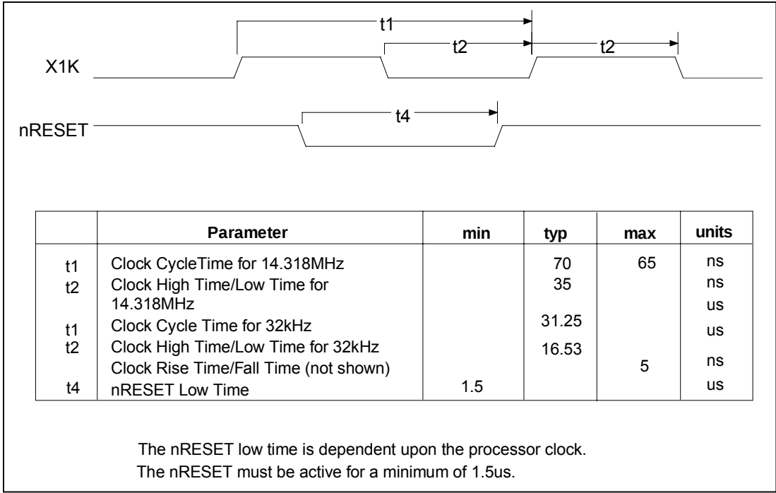
FIGURE 11 - CLOCK TIMING
