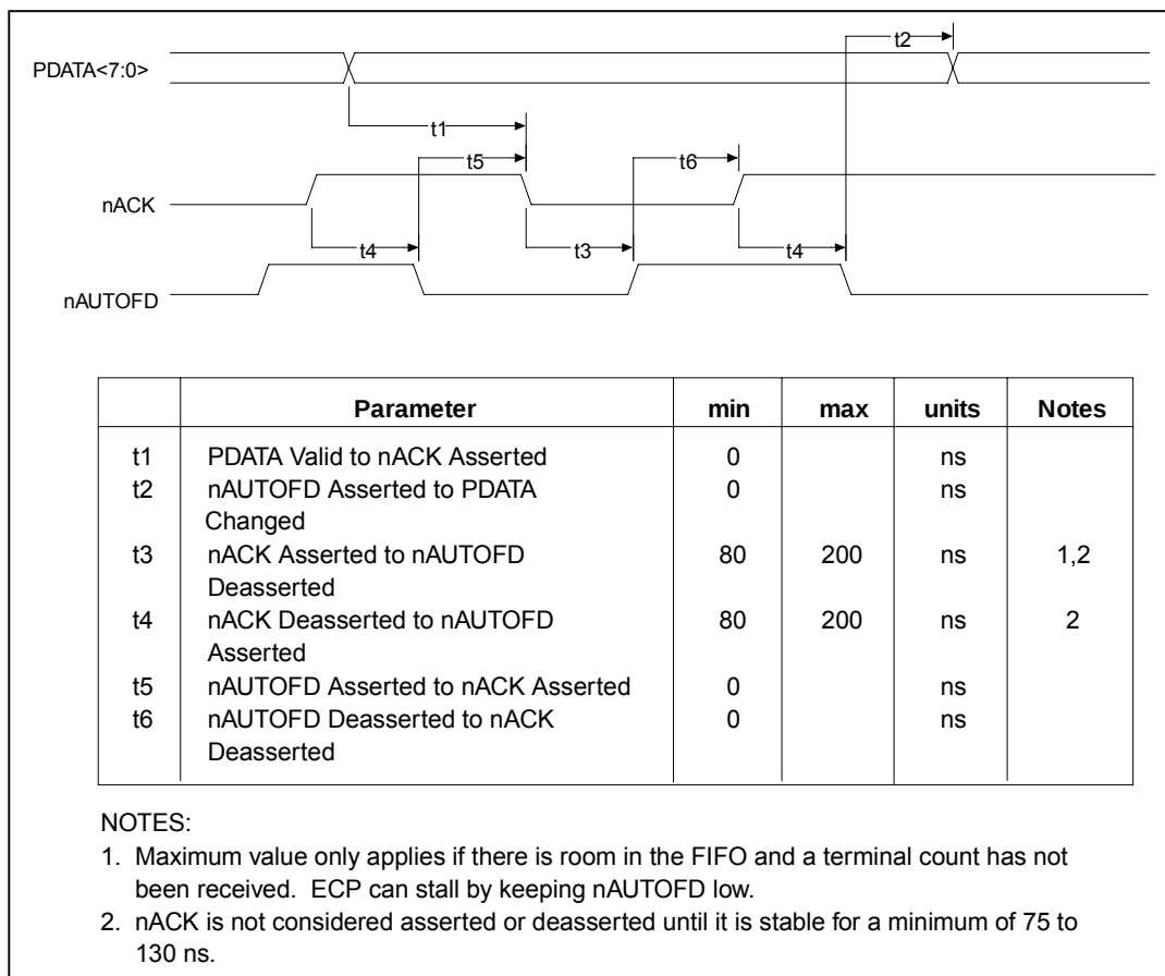
FIGURE 26 - ECP PARALLEL PORT REVERSE TIMING
