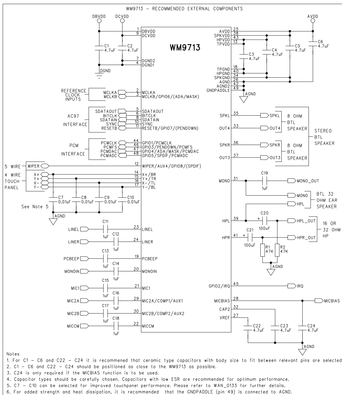
Figure 36 Recommended External Component Diagram
