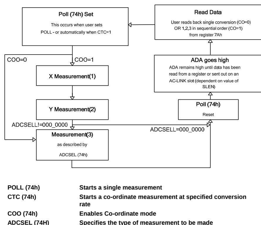
Figure 32 Touchpanel Conversion Flow Diagram
