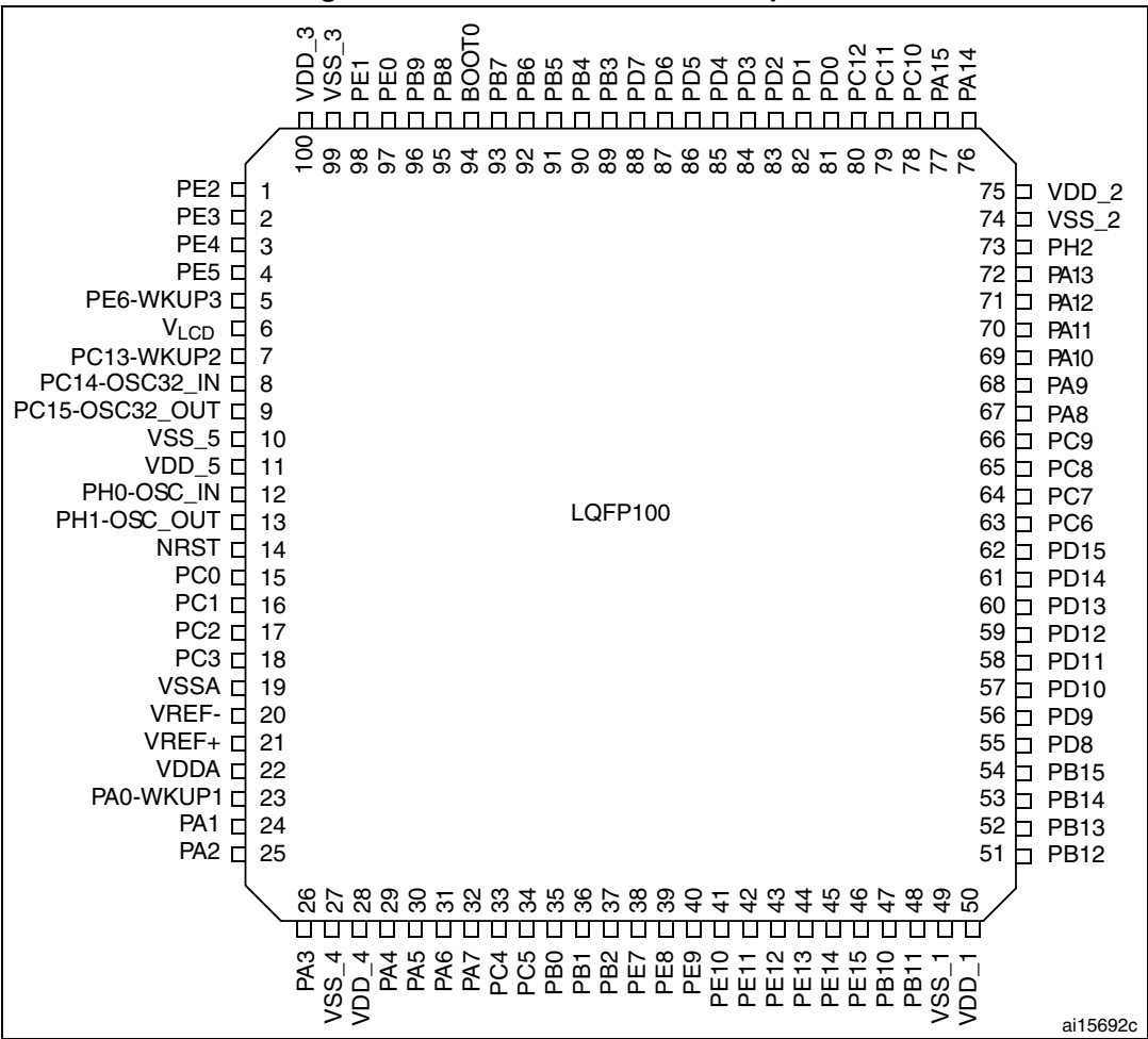
Figure 4. STM32L162VE LQFP100 pinout
