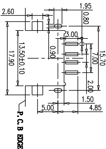
RECOMMENDED P.C.B. PATTERN LAYOUT
