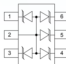
Schematic & PIN Configuration
