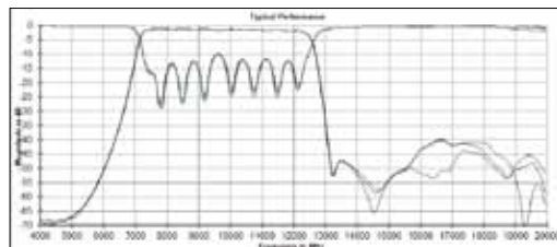
B096QC2S - 8 to 12 GHz
