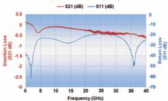
P21BN300MA04733 Opti-Cap Typical Performance (Reference 50 Ohm System)
