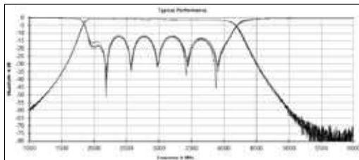
B056RC4S - 4 to 8 GHz
