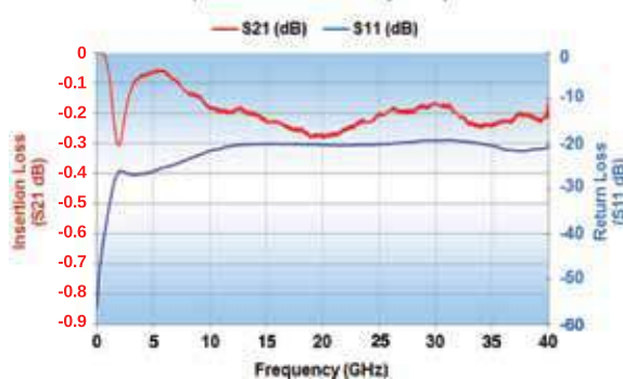
P42BN300MA3182 Opti-Cap Typical Performance (Reference 50 Ohm System)
