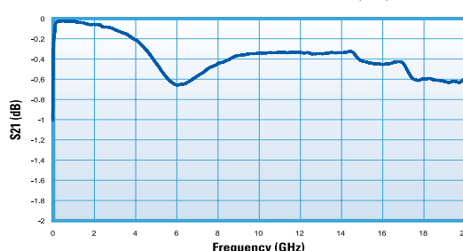
C04BL121X-5UN-X0T Insertion Loss (S21)
