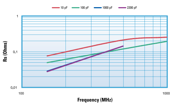
ESR vs Frequency DLI C22 AH Series
