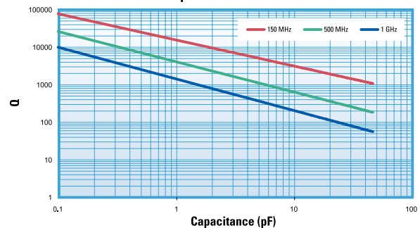
Q vs Capacitance DLI C08 UL Series
