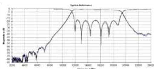
B148QF0S - 12 to 18 GHz
