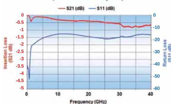
P62BN300MA2636 Opti-Cap Typical Performance (Reference 50 Ohm System)
