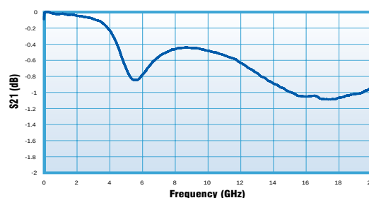
C04BL121X-5UN-X0T Insertion Loss (S21)
