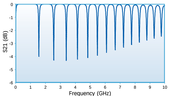
Horizontal Orientation C17AH101K-7UN-X0T 100.0pF Temp = 25°C
