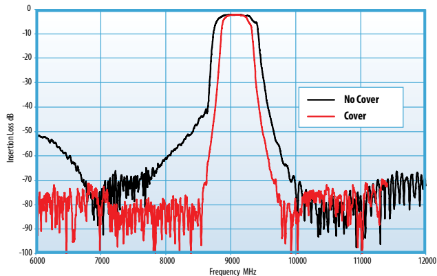
High K substrate provides Higher Field Confinement – 9 GHz Filter (30 mil CF with and without cover).
