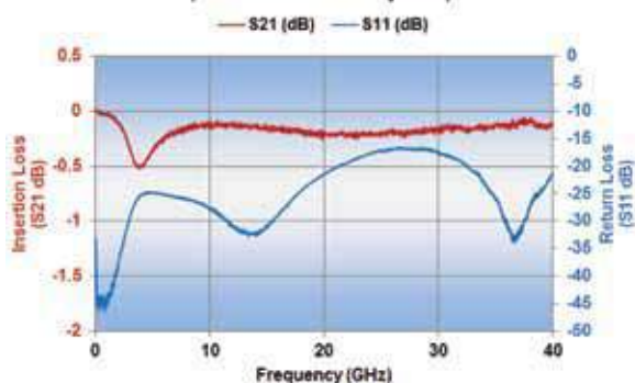
P21BN300MA4572 Opti-Cap Typical Performance (Reference 50 Ohm System)
