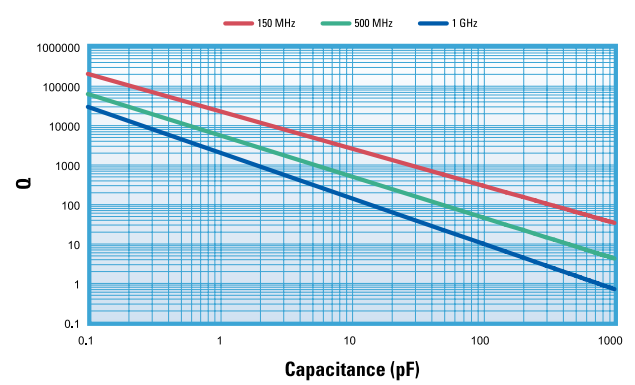
Q vs Capacitance DLI C17 AH Series
