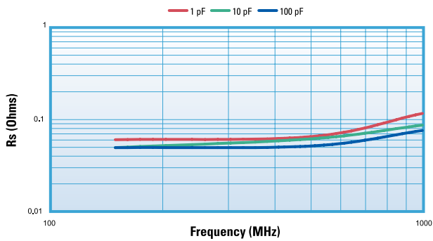
ESR vs Frequency DLI C17 AH Series
