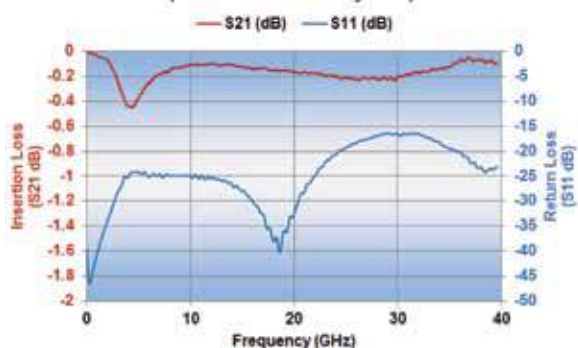
P21BN300MA3976 Opti-Cap Typical Performance (Reference 50 Ohm System)
