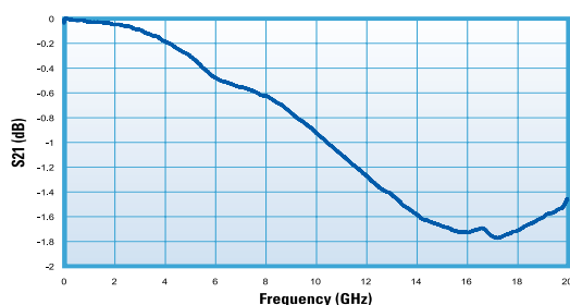
High Q & Broadband MLC Compared Insertion Loss (S21)
