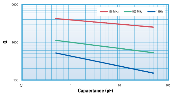
Q vs Capacitance DLI C07 UL Series
