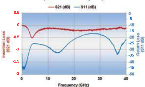
P42BN300MA4679 Opti-Cap Typical Performance (Reference 50 Ohm System)
