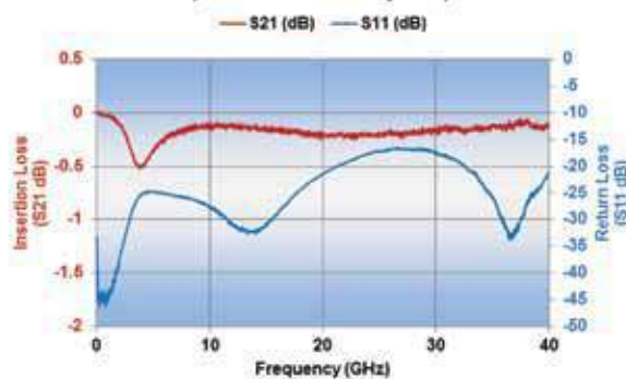
P21BN300MA4282 Opti-Cap Typical Performance (Reference 50 Ohm System)
