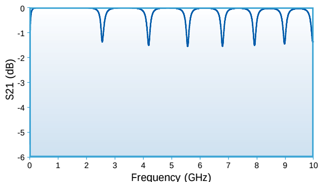
Vertical Orientation C17AH101K-7UN-X0T 100.0pF Temp = 25°C
