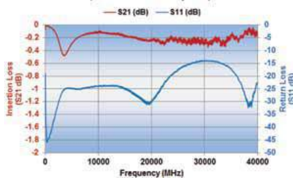
P21BN300MA4678 Opti-Cap Typical Performance (Reference 50 Ohm System)
