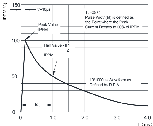
FIG3: Pulse Waveform
