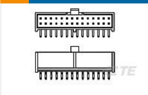
TE Part #1888292-9 FPH-1602G=FLXPAC HDR P 16 RA LF
