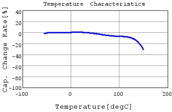
GCJ31CL81E824KA01 C-Temp. capchange, DC0.0V,
