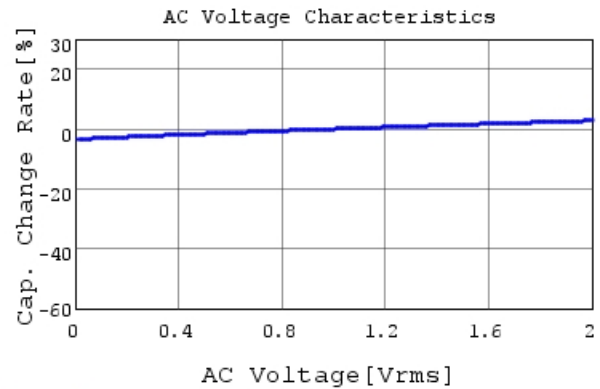
GCJ31CL81E824KA01 C-AC Voltage capchange, Dc
