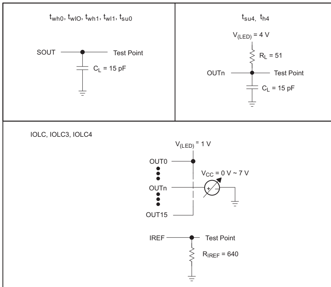
Figure 3. Parameter Measurement Circuits
