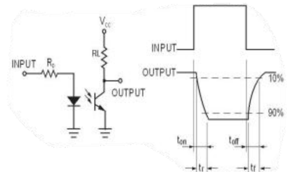
Fig.12 Switching Time Test Circuit & Waveforms
