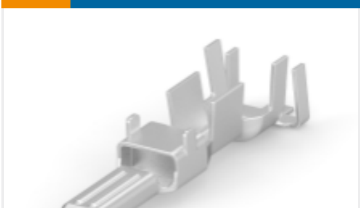
TE Part #4-1971782-2 PTL TAB CONTACT LP, 14 AWG
