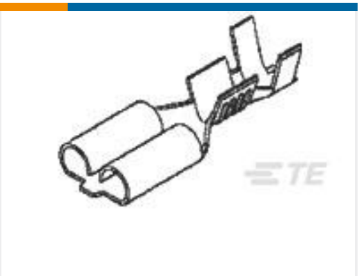
TE Part #170032-2 250 FASTON,REC.,20-14 AWG,BR
