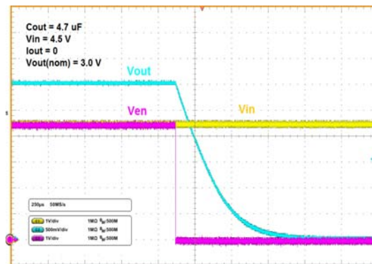
Figure 17. Turn-off by Enable Signal
