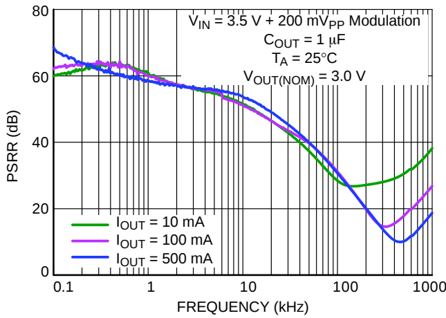
Figure 11. PSRR vs. Frequency & Output Current
