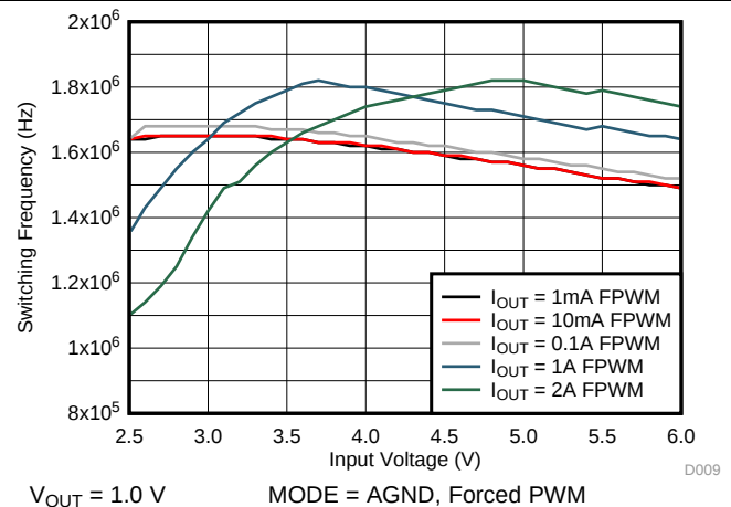
Figure 16. Switching Frequency, Forced PWM Mode (2.0MHz)
