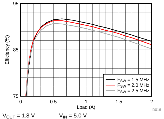
Figure 12. Efficiency with Different Switching Frequency
