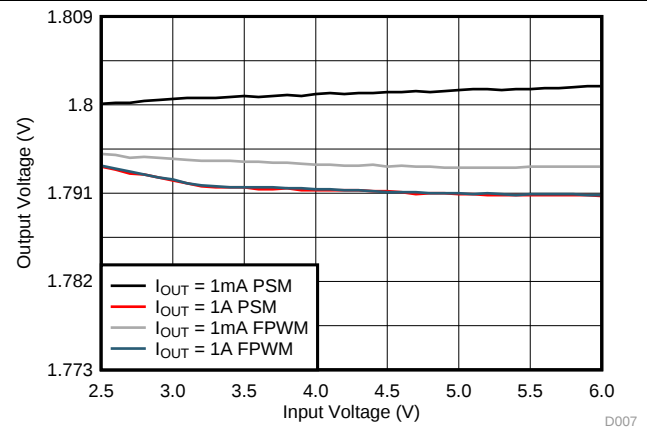
Figure 14. Line Regulation
