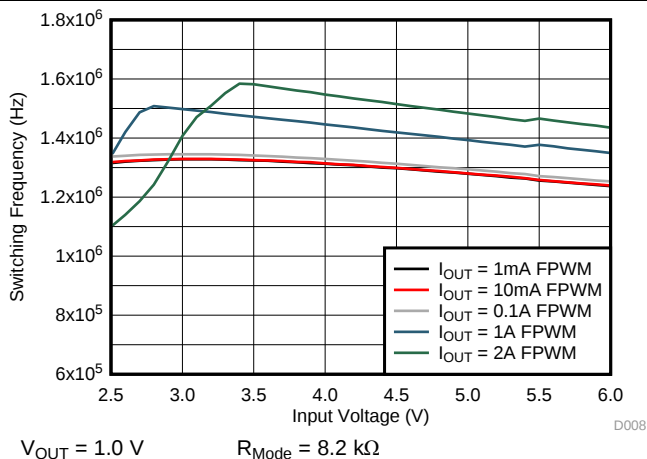
Figure 15. Switching Frequency, Forced PWM Mode (1.5 MHz)
