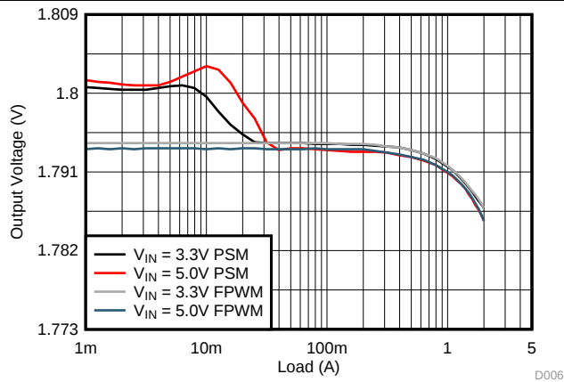
Figure 13. Load Regulation
