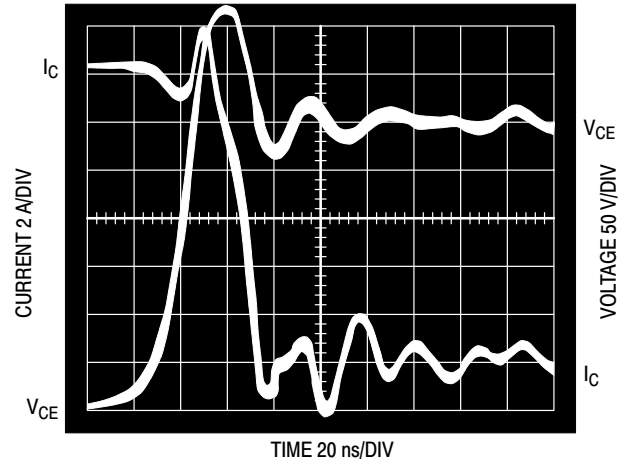
Figure 14. Typical Inductive Switching Waveforms (at 300\text{ V} and 12\text{ A} with I_{B1} = 2.4\text{ A} and V_{BE(off)} = 5\text{ V} )
