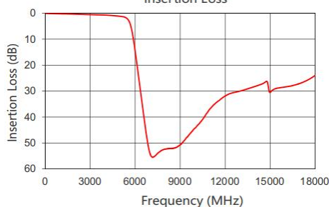
Insertion Loss
