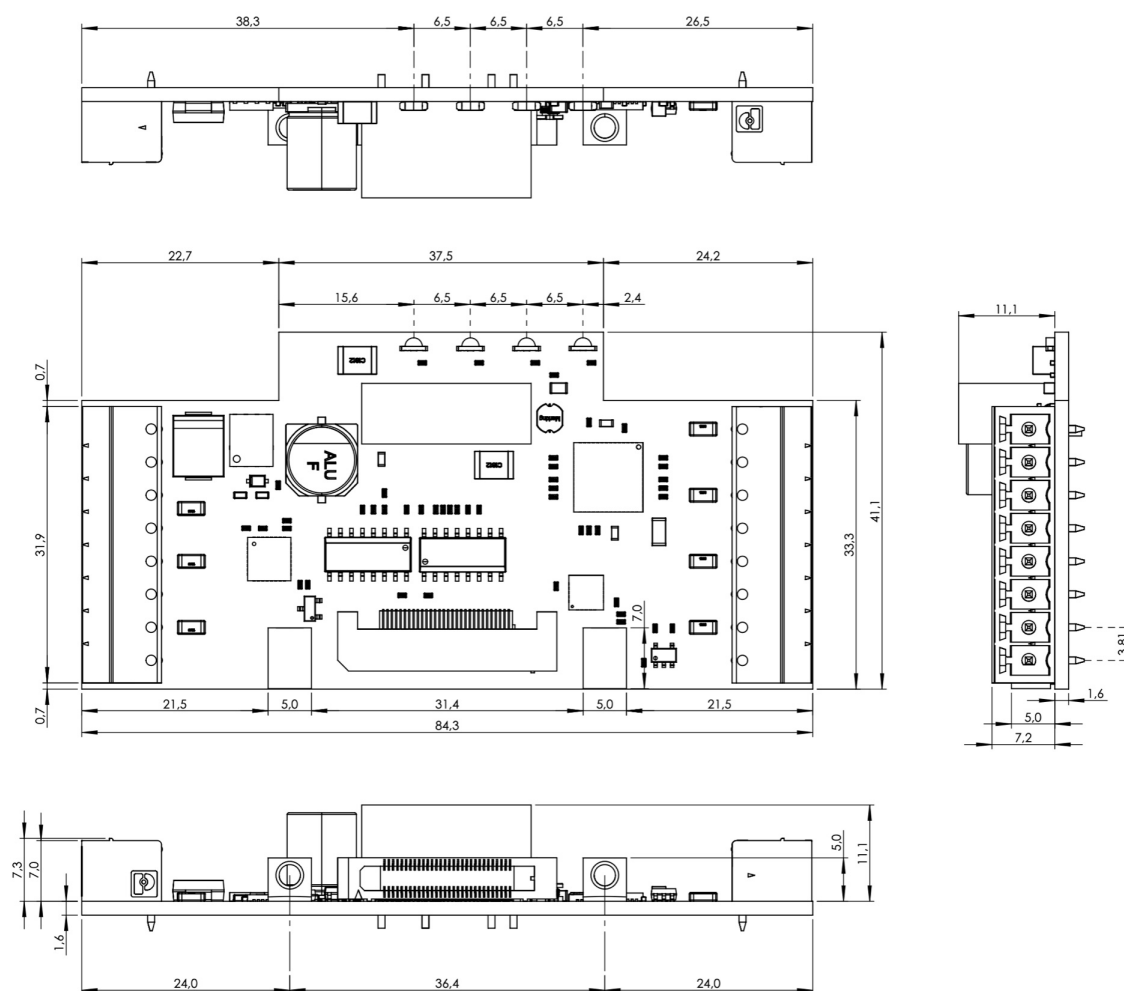
DIMENSIONS (mm)
