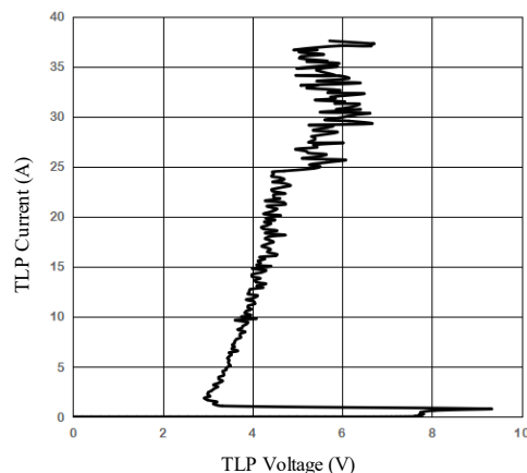
TLP Measurement of I/O to I/O
