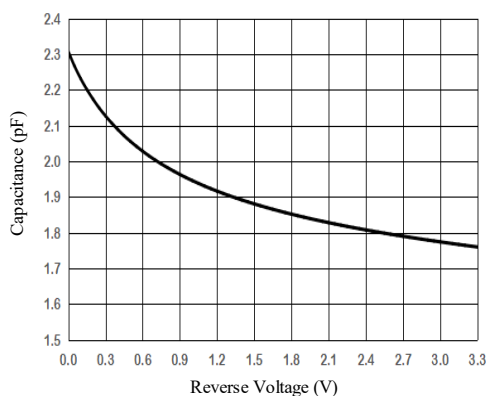
Capacitance vs Reverse Voltage IO to GND
