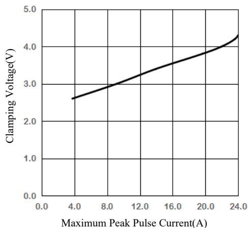
8/20us Current IO to GND
