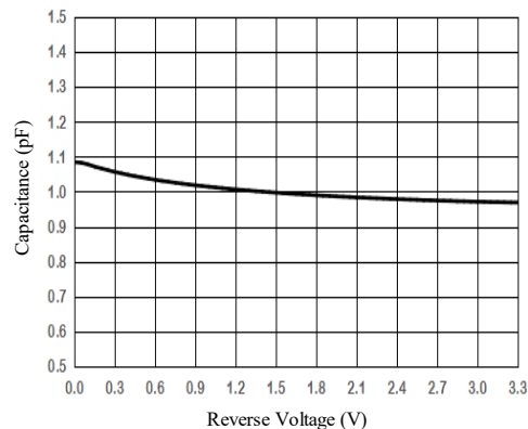
Capacitance vs Reverse Voltage IO to IO
