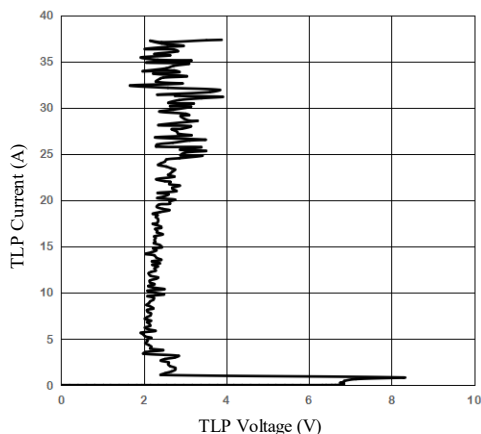
TLP Measurement of I/O to GND
